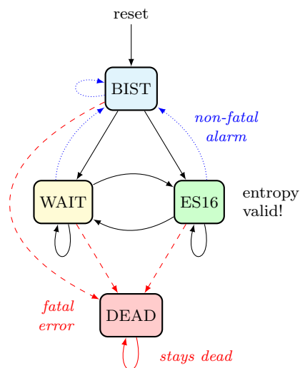
Fig. 2 Normally the operational state alternates between WAIT (no data) and ES16 , which means that a 16-bit random seed has been polled. BIST (Built-in Self-Test) only occurs after reset or to signal a non-fatal self-test alarm (if reached after WAIT or ES16 ). DEAD is an unrecoverable error state. In test mode (when GetNoise / mnoise is active), WAIT and ES16 states are unavailable in the seed CSR.
