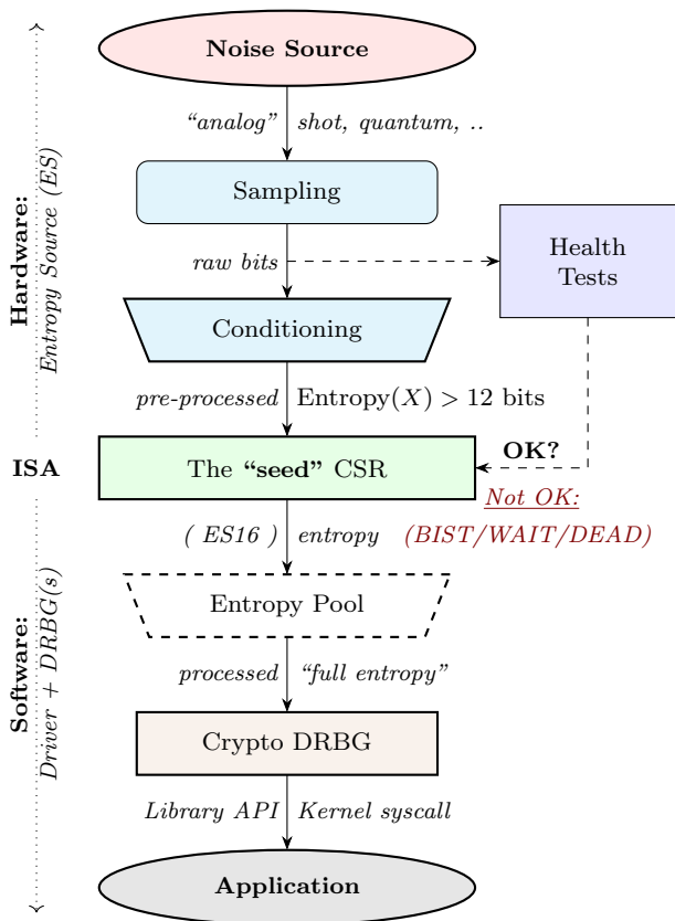
Fig. 1 The seed CSR (Control and Status Register) provides an Entropy Source (ES) only, not a stateful random number generator. As a result, it can support arbitrary security levels. Cryptographic (AES, SHA-2/3) ISA Extension instructions can be used to construct high-speed DRBGs that are seeded from the entropy source.
