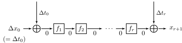
Figure 3: A defective variant of the MALICIOUS framework. Key addition is omitted.
