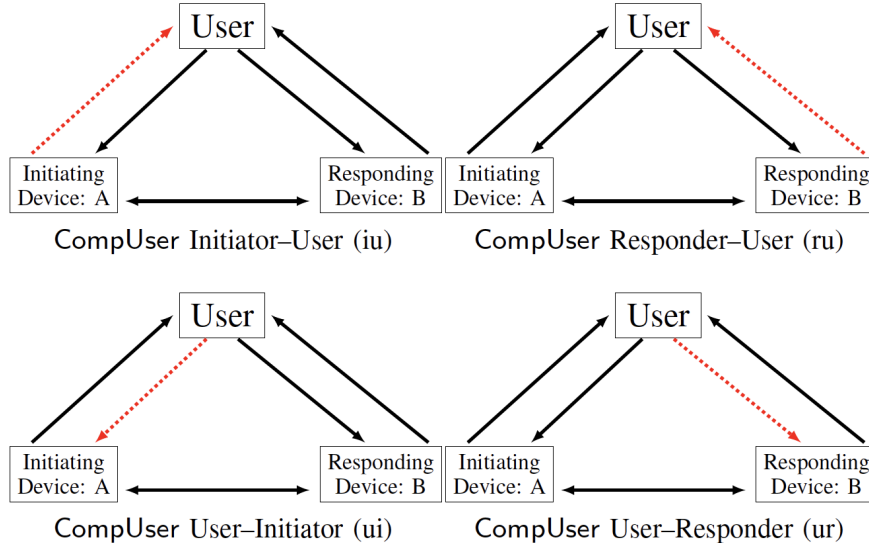
Figure 2: Visual depiction of the baseline four possibilities of user compromise ( CompUser -freshness) where the adversary is allowed to corrupt only one direction of the user-to-device channel at a time, denoted by a red dashed line. We use the abbreviations \text{CompUser}_{[iu]} , \text{CompUser}_{[ru]} , \text{CompUser}_{[ui]} , and \text{CompUser}_{[ur]} to describe the various attack scenarios.
