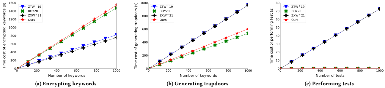
Figure 1: Comparison of Computational Costs with other Lattice-based PEKS Schemes
