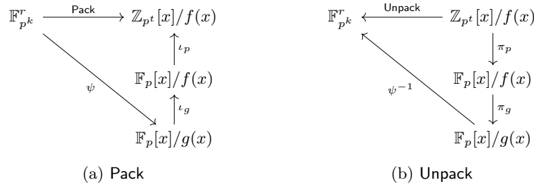
Fig. 6: Definitions of Pack and Unpack in Thm. 6.4
