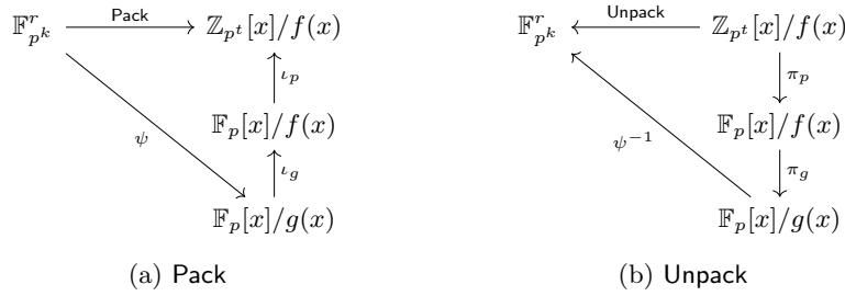
Fig. 8: Definitions of Pack and Unpack in Thm. 7.4
