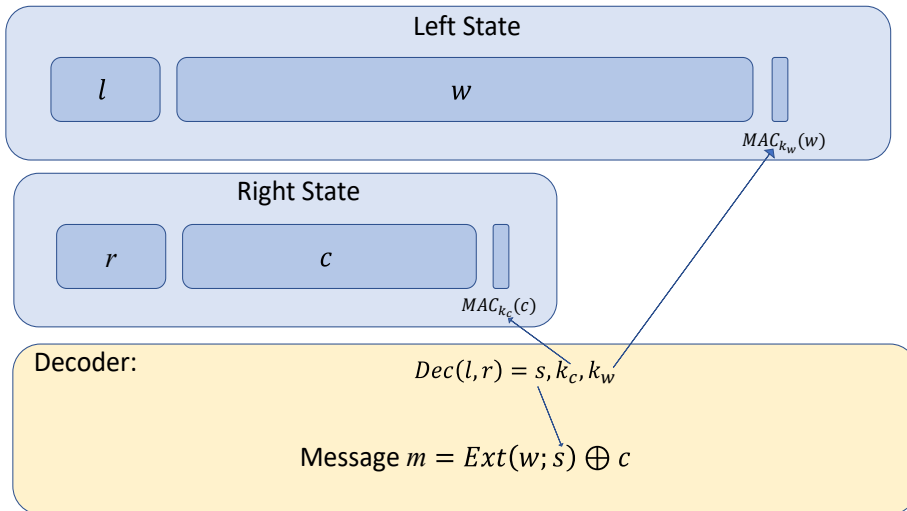
Figure 2: Overview of the construction. Blocks \ell, r come from augmented non-malleable code. The encoder proceeds in steps: first, we randomly sample s, k_w, k_c, w (all independently of the message we are encoding), then we encode s, k_w, k_c using NMC into \ell, r . We then set c = \text{Ext}(w; s) \oplus m , and evaluate \sigma_c as a MAC tag of c on key k_c , and \sigma_w as MAC tag of w on key k_w .
