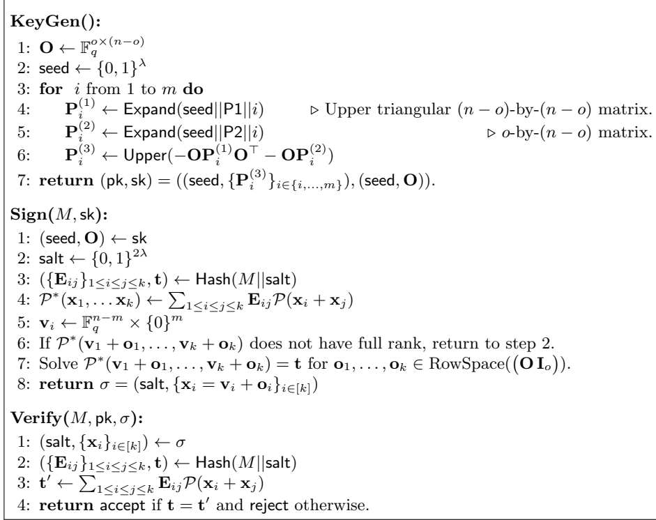
Fig. 2. The key generation, signing, and verification algorithms of the MAYO signature scheme.
