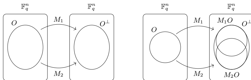
Fig. 1. Behavior of O under M_1 and M_2 , in case n = 2o (on the left) and 2o < n < 3o (on the right).
