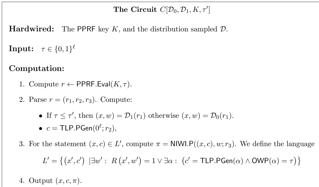
Figure 10: The Circuit C[\mathcal{D}_0, \mathcal{D}_1, K, \tau']
