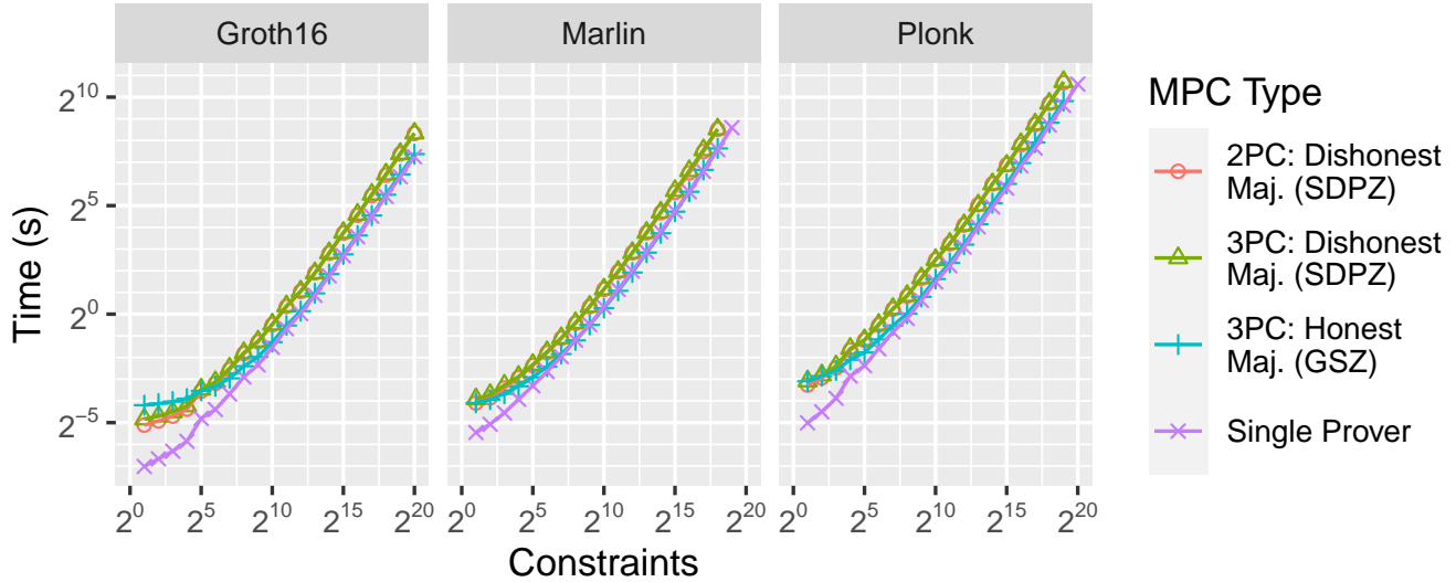
Figure 7: Proving time for varying numbers of parties and protocols, over a 3 gigabit link. MPC denotes a collaboration among N provers. A dishonest majority (SPDZ) protocol is private against <N corrupt provers. An honest majority (GSZ) protocol is private against <N/2 corrupt provers. The baseline is a single prover, using the (non-collaborative) zk-SNARK.
