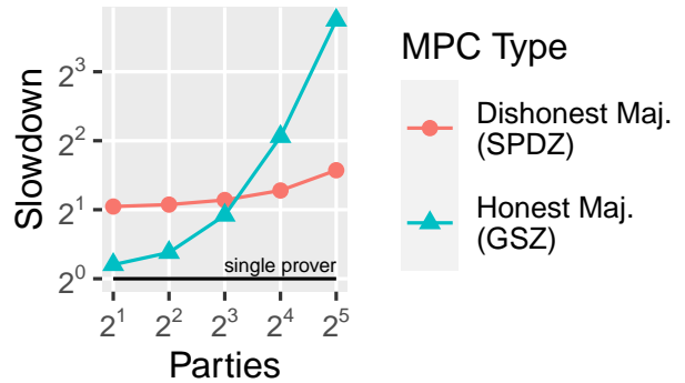
Figure 8: Proving time versus number of parties, normalized by single-prover time. All protocols output Groth16 proofs for 2^{10} constraints over a 3 gigabit link.
