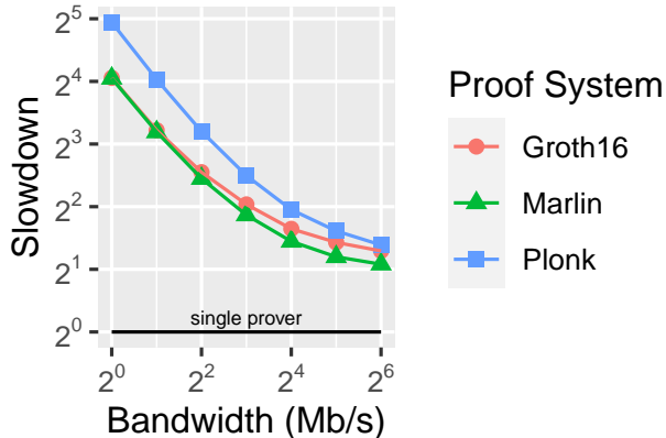
Figure 9: Proving time versus link capacity, normalized by single-prover time. All protocols run with 2 parties, 2^{10} constraints, and the malicious majority protocol (SPDZ).
