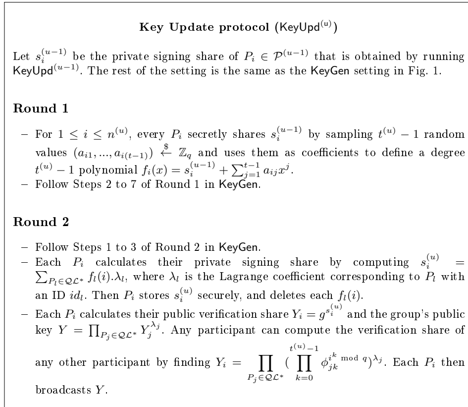
Fig. 4: Key update protocol in ICE FROST
