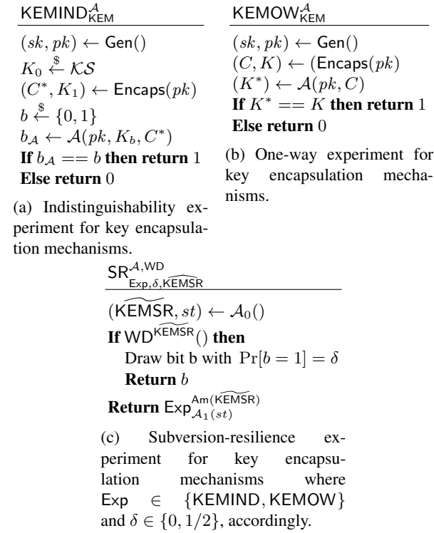
Fig. 4: Security experiments for KEMs.
