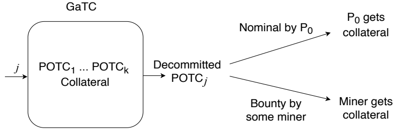
Fig. 1. A GaTC consists of a collection of POTCs with a single associated collateral. The collateral can be transferred to the party that opens the desired POTC, either P_0 through the nominal path or a bounty hunter. The index j indicates which POTC to open.
