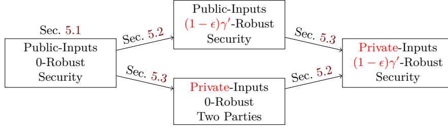
Fig. 2. Gage MPC. The fully private input versions are for two parties only.
