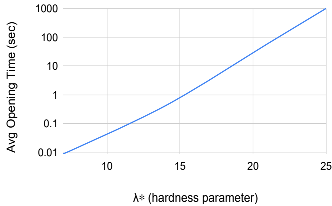
Fig. 3. Impact of capsule difficulty (i.e., \lambda^* ) on the average opening time. Note the y-axis uses a logarithmic scale to capture the exponential relationship.
