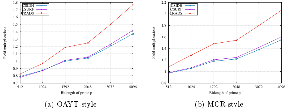
Fig. 1: Running time regarding the group action evaluations of CSIDH, CSURF, and CRADS. The numbers are given in millions of multiplications, and they correspond with the average of 1024 random instances.
