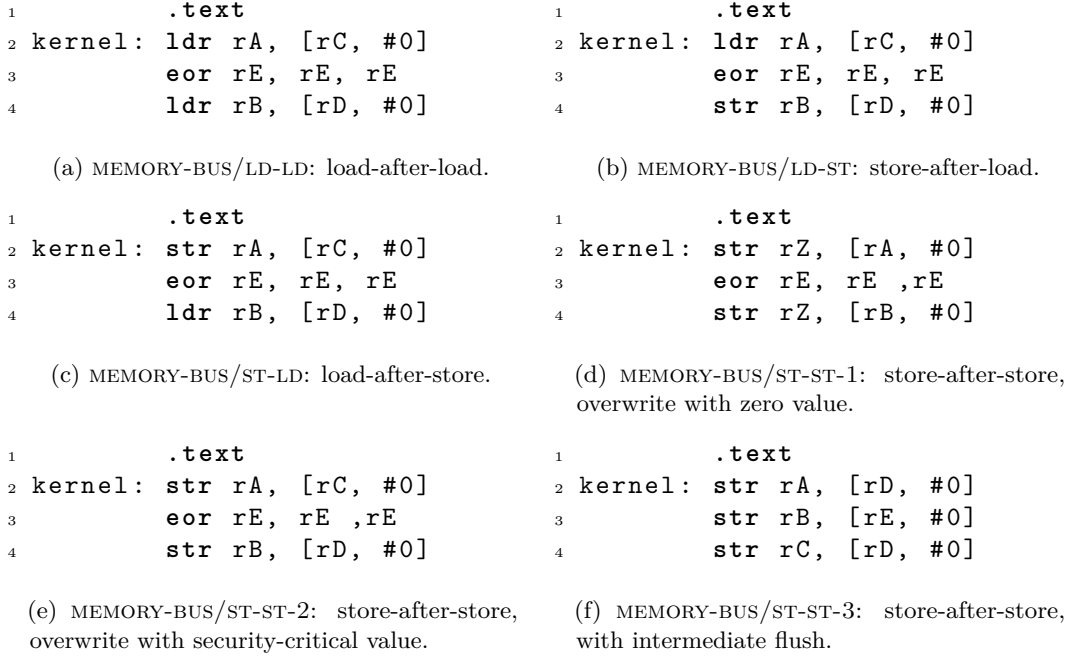
Figure 3: Pseudo-code for micro-benchmarks described in Section 5.1.1, i.e., those related to the case study on hidden state in the memory access path.
