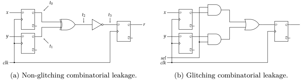
Figure 1: Two example designs, illustrating the difference between non-glitching combinatorial leakage and glitching combinatorial leakage. In the top design, only combinatorial leakage is evident, based on how the signals t_0 and t_1 change on each clock cycle; subsequent signals, e.g., t_2 and t_3 , change only once per clock cycle. Note this ignores the effect of wire delay on t_0 and t_1 . In the bottom design (a multiplexer), if the sel , x , and y signals all change, then the delayed sel signal will cause Hamming distance leakage on r : this causes it to glitch, i.e., change multiple times per clock cycle.
