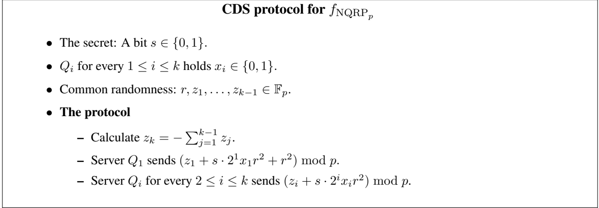
Figure 1: A k -server CDS protocol with Degree-3 Encoding for f_{\text{NQR}_p} .
