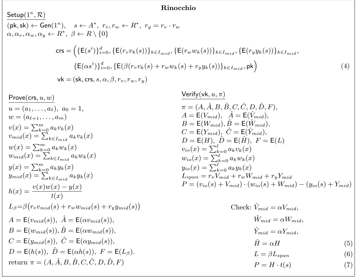
Fig. 1. The Rinocchio scheme for (zk-)SNARKs over a ring R .
