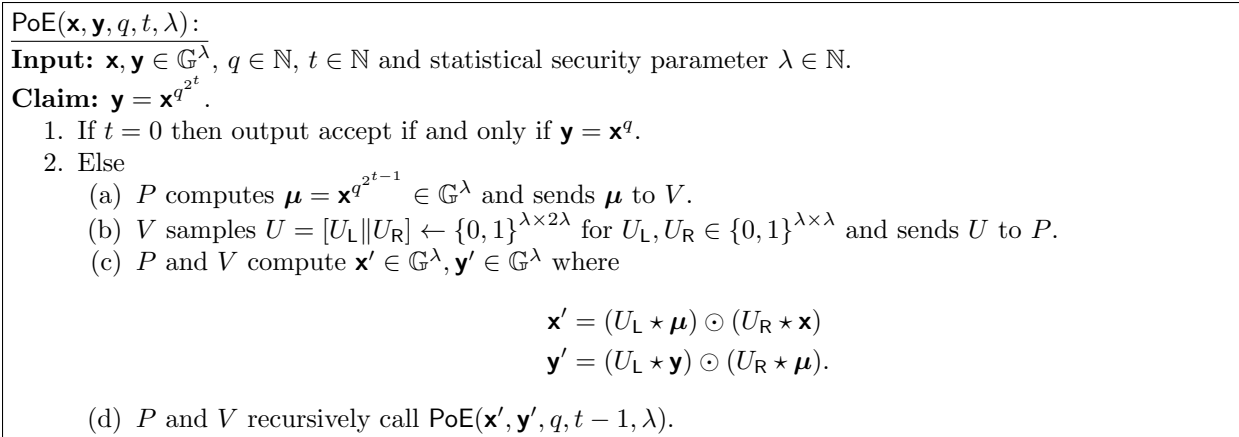
Figure 1: Proof-of-Exponentiation Protocol
