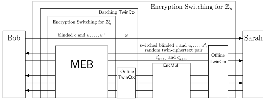
Fig. 7: Packing Encryption Switching Procedure for \mathbb{Z}_n Case
