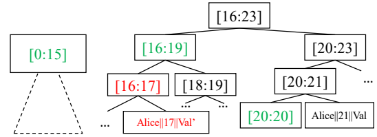
Fig. 5: Alice appends the first value \text{Val} for her ID at position 21. Someone (either another honest user or the attacker) has appended \text{Val}' for ID “Alice” at position 17 already. Alice will verify the first-value proof, which contains non-membership proofs for ID “Alice” in the prefix trees at the green nodes.
