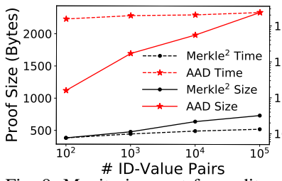
Fig. 9: Monitoring cost for auditors in AAD and Merkle 2 .
