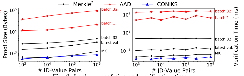
Fig. 8: Lookup proof size and verification time.
