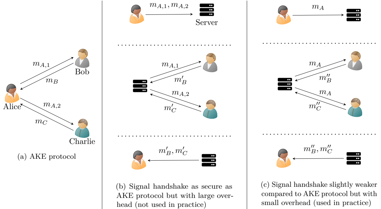
Figure 3: Comparison of the message flow of an AKE protocol (left) and that of a Signal handshake (center and right). The center protocol is more secure than the right protocol, while the right protocol is storage and bandwidth efficient compared to the center. The implemented Signal protocol uses the right protocol.
