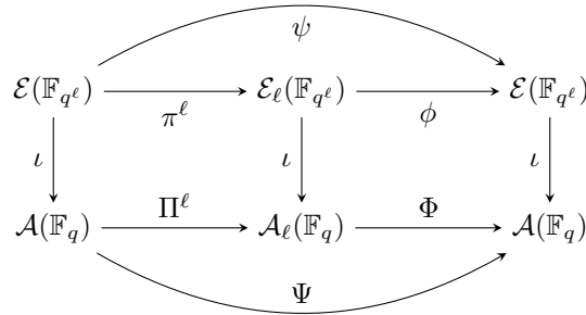
Figure 1: Endomorphism diagram
