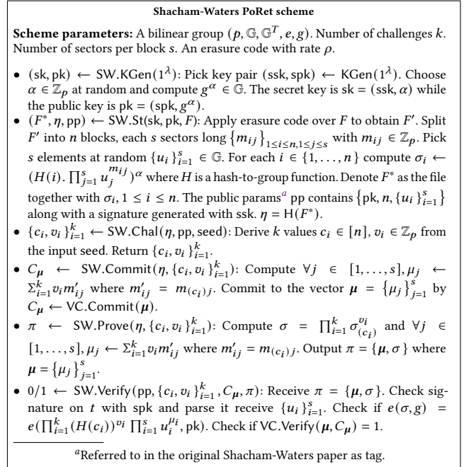
Figure 6: The Shacham-Waters PoRet scheme with an extra commitment step.
