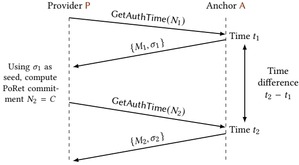
Figure 3: The geo-commitment protocol.
