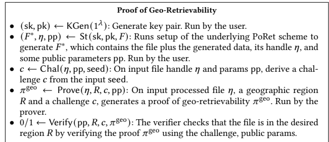
Figure 1: API of a PoGeoRet scheme.
