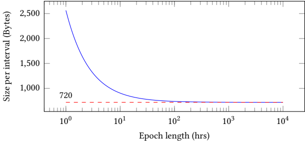
Figure 4: For a fixed interval length of 1hr, the proof size per interval for GoAT (vs) the epoch length. Roughtime anchor.
