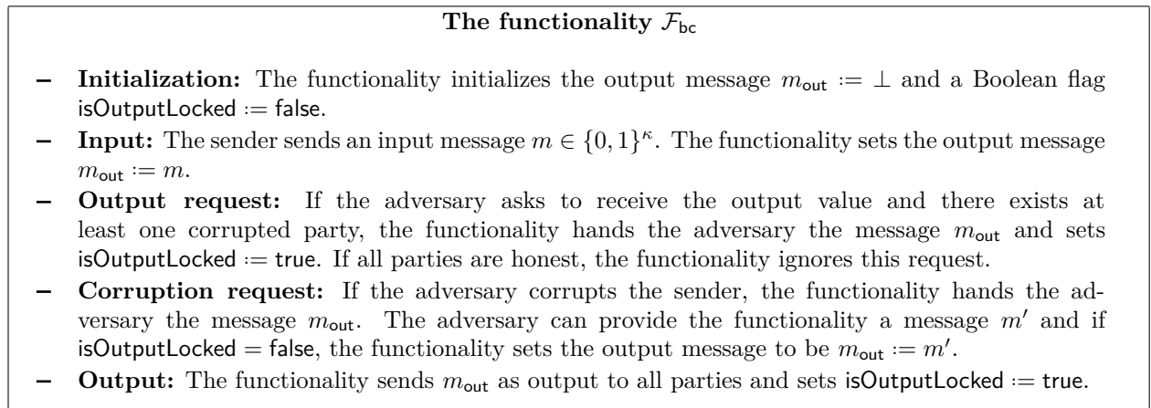
Figure 2: The broadcast functionality
