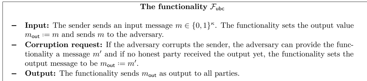
Figure 3: The corruption-unfair broadcast functionality
