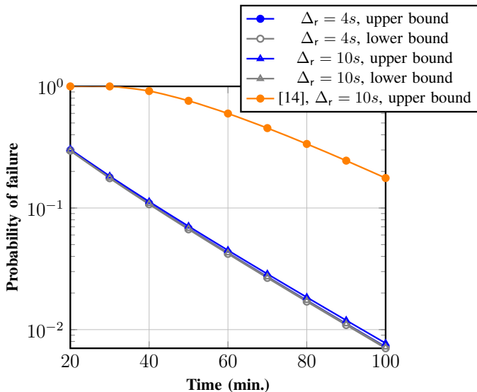
Figure 3. Bitcoin temporal settlement failure for a 10% adversary, results from [14] for comparison.
