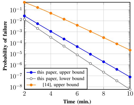
Figure 2. Our upper and lower bounds on settlement failure probability for Ethereum with a 10% adversary and 2 second network delays; results from [14] included for comparison.
