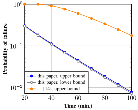
Figure 1. Our upper and lower bounds on settlement failure probability for Bitcoin with a 10% adversary and 10 second network delays; results from [14] included for comparison
