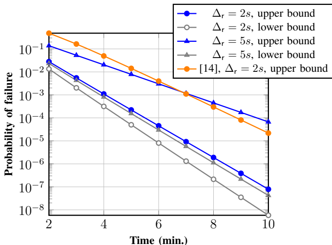
Figure 4. Ethereum temporal settlement failure for a 10% adversary, results from [14] for comparison.
