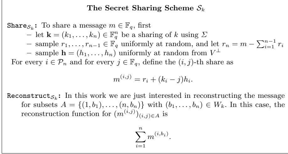
Fig. 4. The \mathbb{F}_q -LSSS \mathcal{S}_k related to the secret sharing scheme \Sigma , the affine subspace W_k = [k]_\Sigma , and V = [0]_\Sigma .
