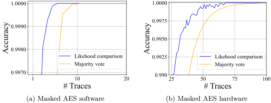
Figure 1: Oracle accuracy using majority vote and likelihood comparison.
