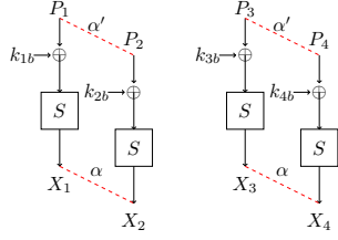
Fig. 3: Nonlinear relations in key-recovery phase.
