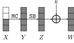
Fig. 18: Reducing complexity of \varepsilon .
