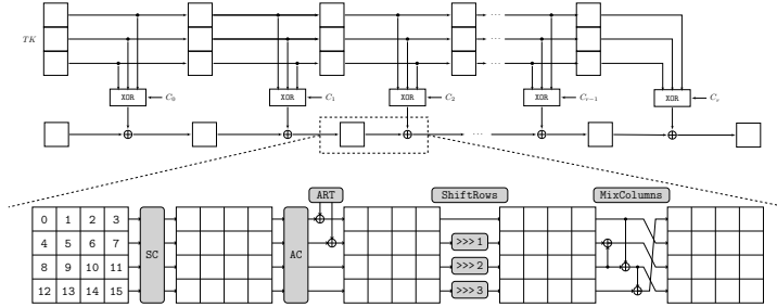
Fig. 10: The framework of SKINNY- n-3n . (Thanks to https://www.iacr.org/authors/tikz/ )
