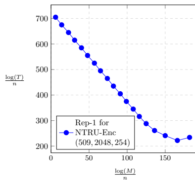
Fig. 2: Time-memory tradeoffs
