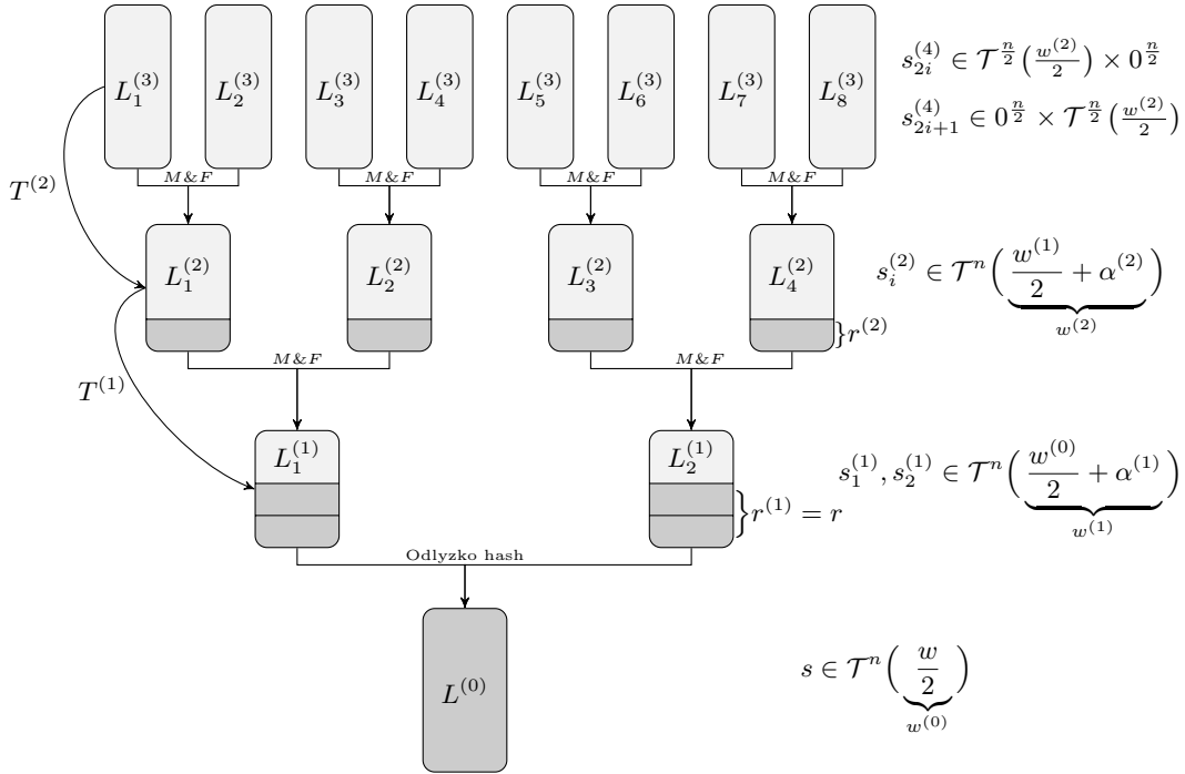
Fig. 1: The classical MEET-LWE algorithm
