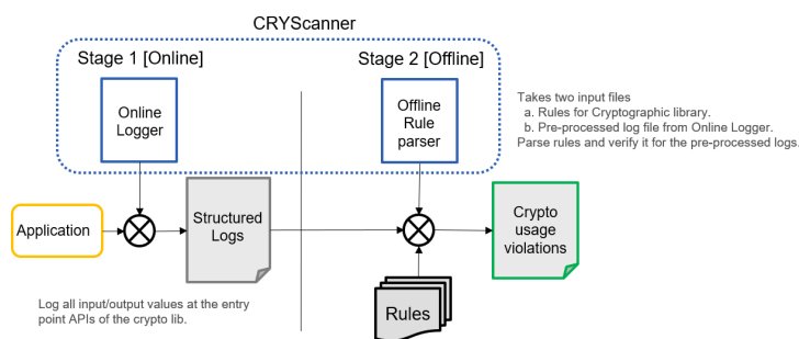
Fig. 3. CRYScanner execution flow diagram
