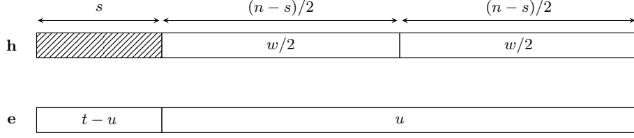
Figure 4.1. The form of the parity-checks produced by this method, vs. the bet made on the error. The hatched rectangle of size s for \mathbf{h} indicates that the weight is arbitrary on this part.
