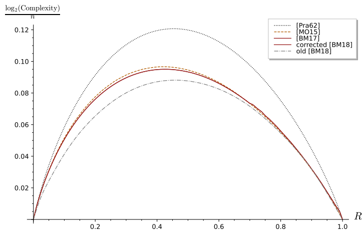
Fig. B.1. Corrected complexity of the [BM18] decoder.
