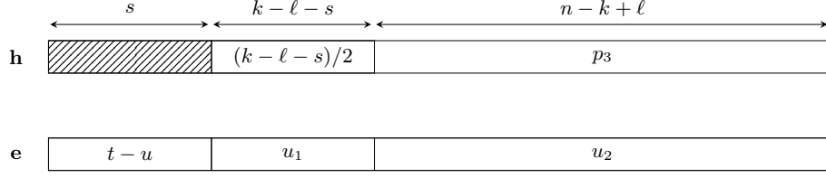
Fig. 5.2. The form of the parity-checks produced by this method [BJMM12], vs. the bet made on the error. The hatched rectangle of size s for \mathbf{h} indicates that the weight is arbitrary on this part.
