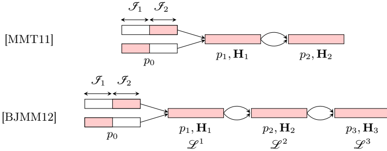
Fig. 5.1. This figure represents the successive lists obtained in [MMT11] and [BJMM12]. The support of the elements of the list are represented in pink. Arrows point from the lists which are merged to the result of the merge and if two arrows depart from a list and arrive at another list, this means that the departure list is merged with itself. The weights of the elements are indicated for each level and the matrix \mathbf{H}_i used for the merge is also given at the level of the result of the merge.
