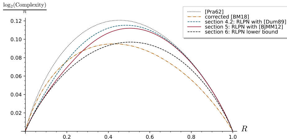
Fig. 6.1. Complexity exponents of our different RLPN decoders, ISD's and the genie-aided RLPN algorithm when splitting parity-checks in two parts.
