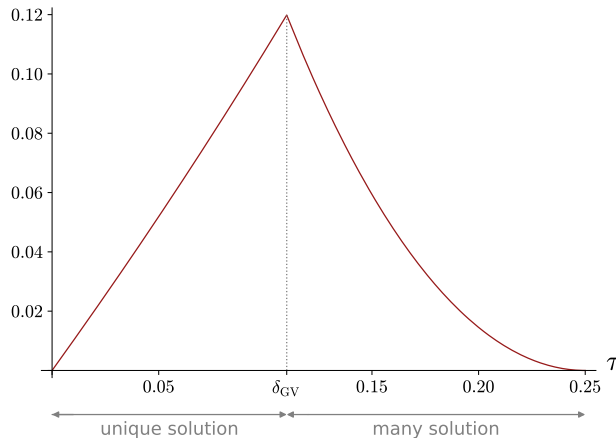
Fig. 1.1. Complexity exponent \alpha of the Prange ISD algorithm [Pra62] as a function of the error ratio \tau \triangleq \frac{t}{n} at rate R = \frac{1}{2} . The peak corresponds to the normalized Gilbert-Varshamov distance \delta_{\text{GV}} = h^{-1}(1 - R) .
