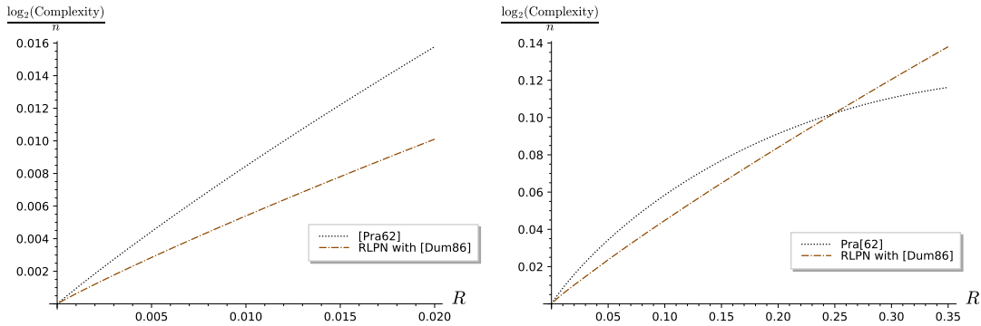
Fig. 4.2. The complexity of the RLPN-decoder for very small rates vs. the simplest information set decoder, namely the ISD Prange decoder [Pra62]. For small R , there is not much difference between the ISD Prange decoder and much more evolved decoders like [BJMM12, MO15, BM17, BM18]. The RLPN-decoder with the very simple [Dum86] technique performs much better for small rates than ISD decoders. It is only outperformed by the Prange decoder for rates above 0.25 approximately.
