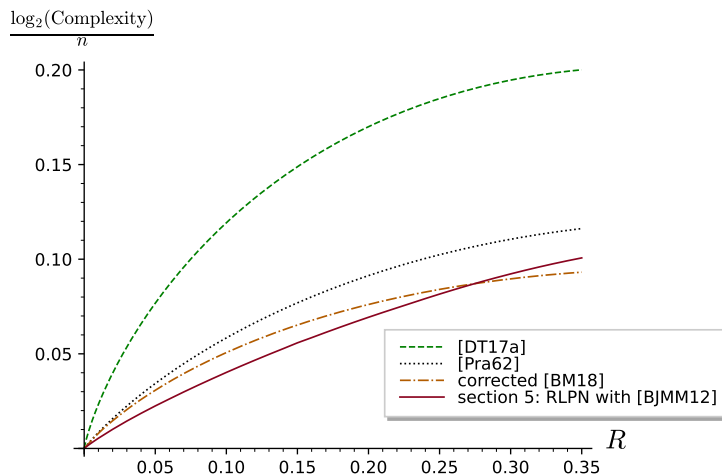
Fig. 1.2. Complexity exponent for full distance decoding of genie-aided statistical decoding [DT17, §7] (recall that this is a lower bound on the complexity exponent of statistical decoding), the basic Prange ISD algorithm [Pra62], the best state-of-the-art algorithm of [BM18] (with a correction in the exponent that we give here, see Appendix B) and our RLPN decoder as a function of R .
