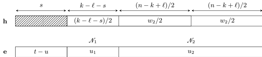
Fig. 4.3. The form of the parity-checks produced by this method, vs. the bet made on the error. The hatched rectangle of size s for \mathbf{h} indicates that the weight is arbitrary on this part.
