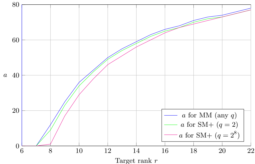
Fig. 4. Optimal values of a with m = n = 200, k = 100, q = 2 or q = 2^8 , for \text{MM-}\mathbb{F}_q and \text{SM-}\mathbb{F}_{q^m}^+ .
