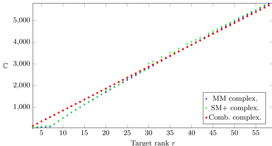
Fig. 1. Comparison between the theoretical complexities \mathbb{C} of MM- \mathbb{F}_q /SM- \mathbb{F}_{q^m}^+ (the best one, hybrid and punctured version) and of the combinatorial attack for RD instances with fixed (m, n, k) = (200, 200, 100) and various values of r . The rank Gilbert-Varshamov bound is d_{\text{RGV}}(m, n, k, q = 2) = 58 .
