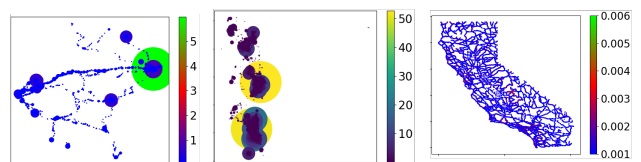
Figure 5: (Left) SPITZ, (Middle) GOWALLA, and (Right) CALI datasets on domain 2^{10} \times 2^{10} . The color map (and relative size of the markers) indicate the number of records (in thousands) on each domain point.
