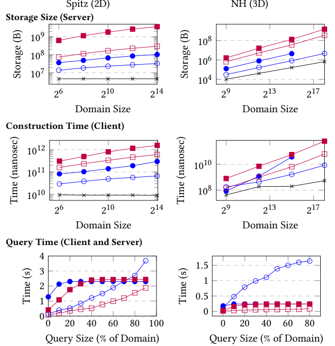
Figure 8: Storage size and construction time of the schemes by domain size on SPITZ (28,837 records) and NH (number of records n = m^{2/3} , where m is the domain size), with logarithmic scale on the y-axis. Query time of the schemes by query size on SPITZ (28,837 records in domain [2^{10}] \times [2^{10}] ) and NH (4096 records in domain [2^6] \times [2^6] \times [2^6] ).
