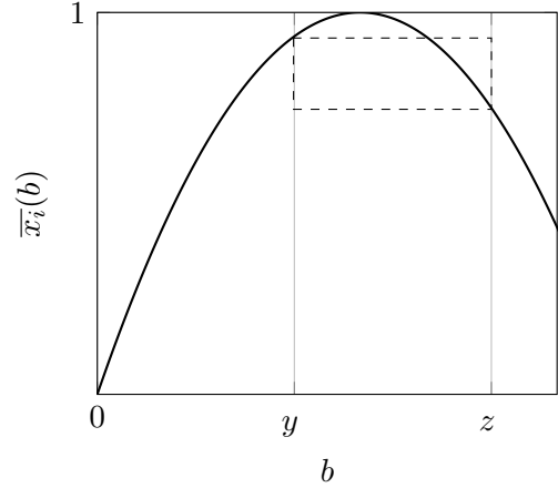
(b) When the function decreases, S(y, z) can be negative. S(y, z) is the negative of the dashed rectangle area.
