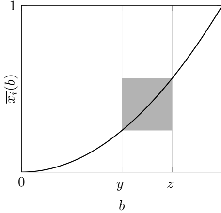
(a) An illustrative example of S(y, z) in increasing function. The size of the gray area in the figure is exactly S(y, z) .
