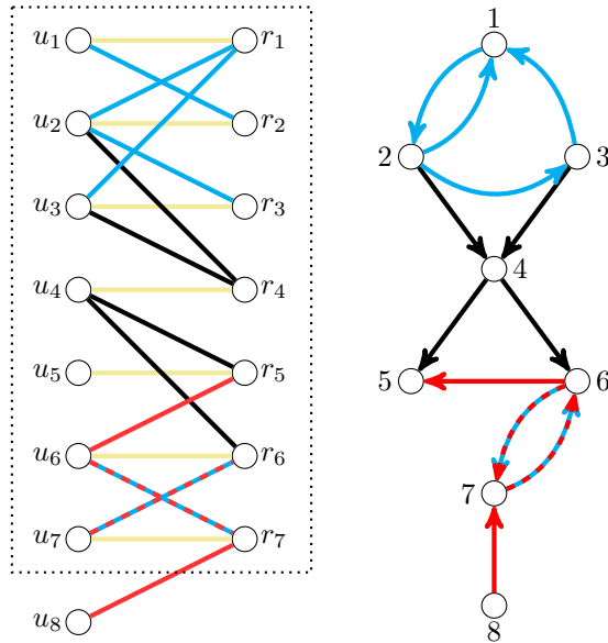
Figure 2: Example of a transaction graph G ( U and R being nodes on left and right respectively) and its induced digraph \text{id}(G) . The subgraph in the dotted rectangle is G^\alpha . The yellow, blue and red edges correspond to edges considered in Lemma 4.1 Item 1 to Item 3 respectively, the black edges are none of them.
