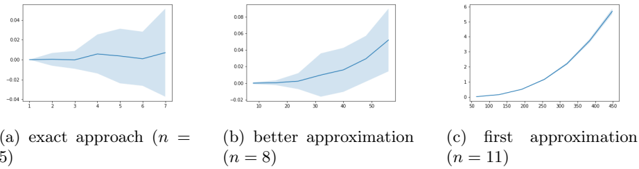
Fig. 5: Results of simulations: difference of the logarithm of the results between simulation and conjectural prediction by number of equations (line is mean over 100 tries, area is variability)
