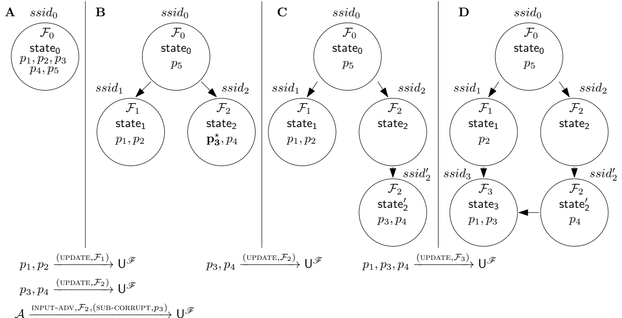
Figure 3: Example of an execution of \mathcal{U}^{\mathcal{F}} (we dropped \text{StUp} and \text{UpPred} to not overburden the notation).
