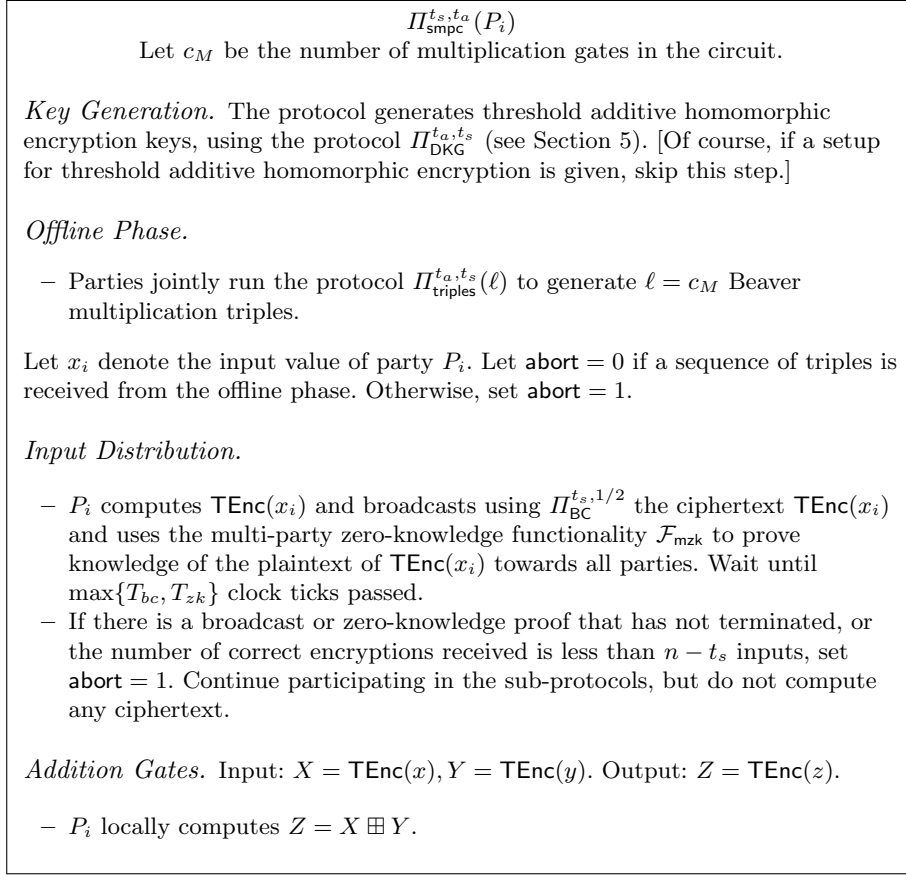
Fig. 14: Synchronous MPC with unanimous output (part 1).
