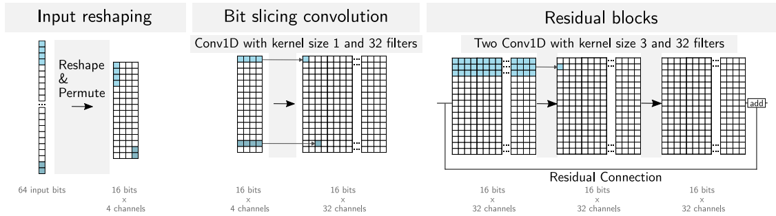
Figure 1: Visualization of three main parts of Gohr’s neural distinguisher.
