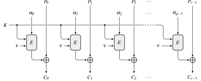
Figure 5: CounTeR in Tweak mode
