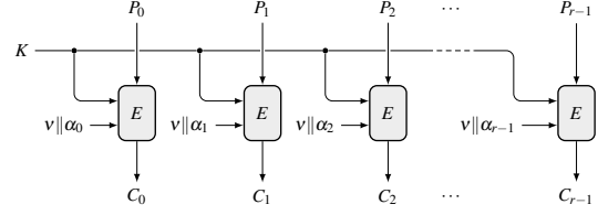
Figure 4: Tweaked ECB mode
