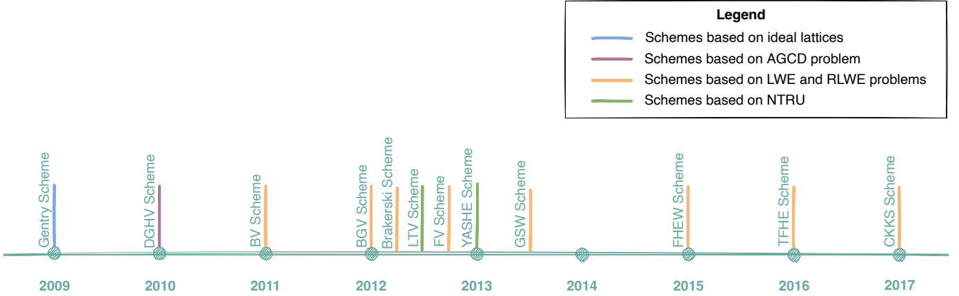
Fig. 2. Timeline of the main FHE schemes.
