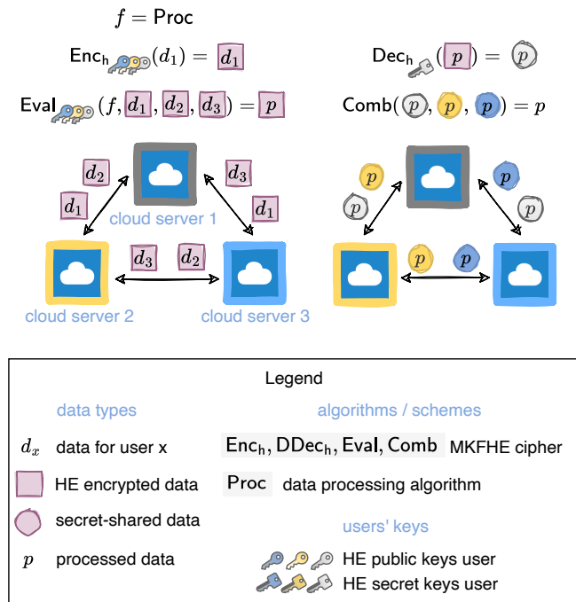
Fig. 16. MPC constructed with MKFHE. Only the operations performed by cloud server 1 have been detailed in the figure, but the rest of the parties behave analogously. For simplicity, the algorithm \text{Enc} in the figure generates a ciphertext for multiple keys, but in [273] this is achieved with an Expand algorithm.
