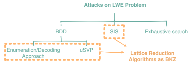
Fig. 11. Different solving approach to LWE problem
