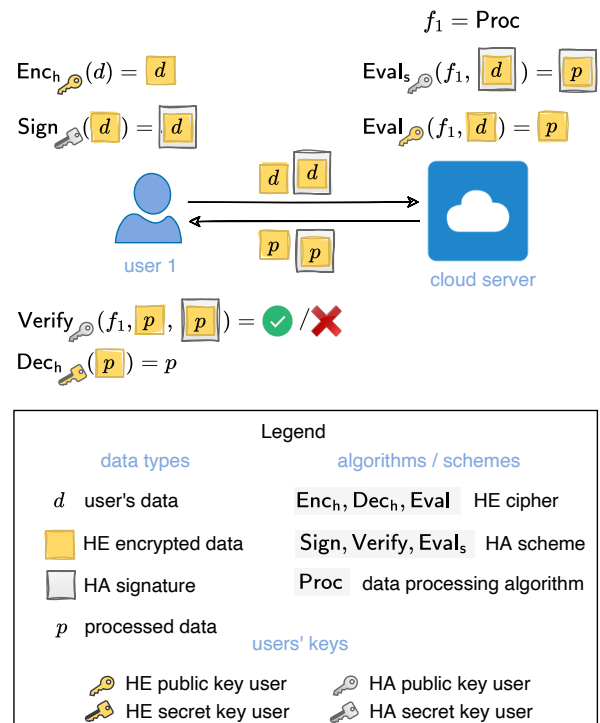
Fig. 15. FHAE by composition encrypt-then-sign.
