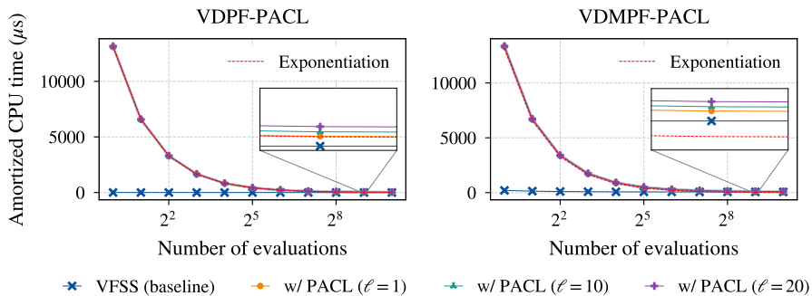
Fig. 6: Our VDPF-PACL construction is dominated by the exponentiation in \mathbb{F}_p^* (dashed lined) and has a higher initial overhead compared to the DPF-PACL construction. In contrast to DPF-PACLs, our VDPF-PACL construction amortizes almost entirely after 64 evaluations and has an asymptotically smaller overhead.
