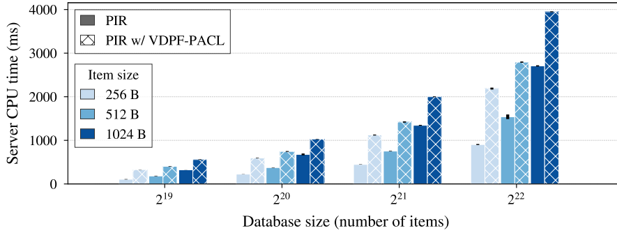
Fig. 6: Server-side CPU time for privately retrieving an item from a database through two-server PIR with and without VDPF-PACLs. Adding access control has a 1.5–3× impact on processing time. The access control overhead is automatically amortized over the number of items in the database. The relative overhead also diminishes as the items in the database become larger.
