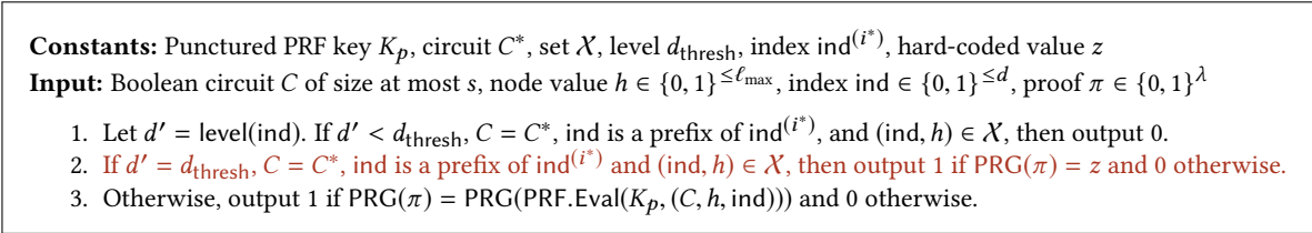
Figure 13: Program \text{Prove}''[K_p, hk, C^*, \mathcal{X}, d_{\text{thresh}}, \text{ind}^{(i^*)}, z]
