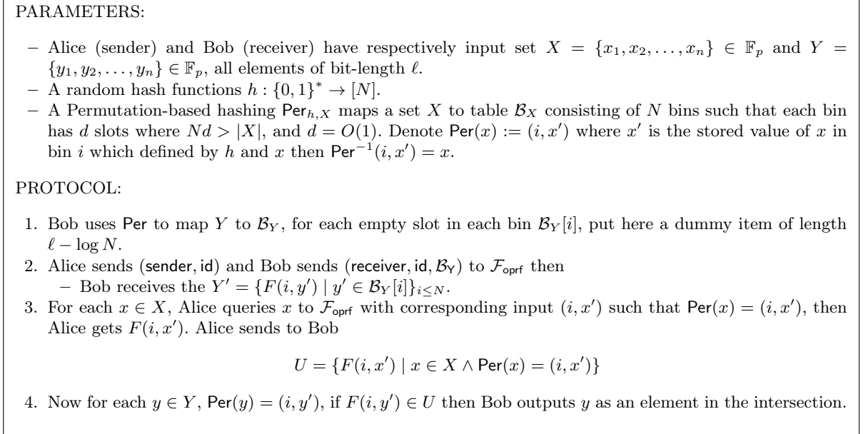
Fig. 5. Our malicious PSI protocol based on \mathcal{F}_{\text{opr}}f
