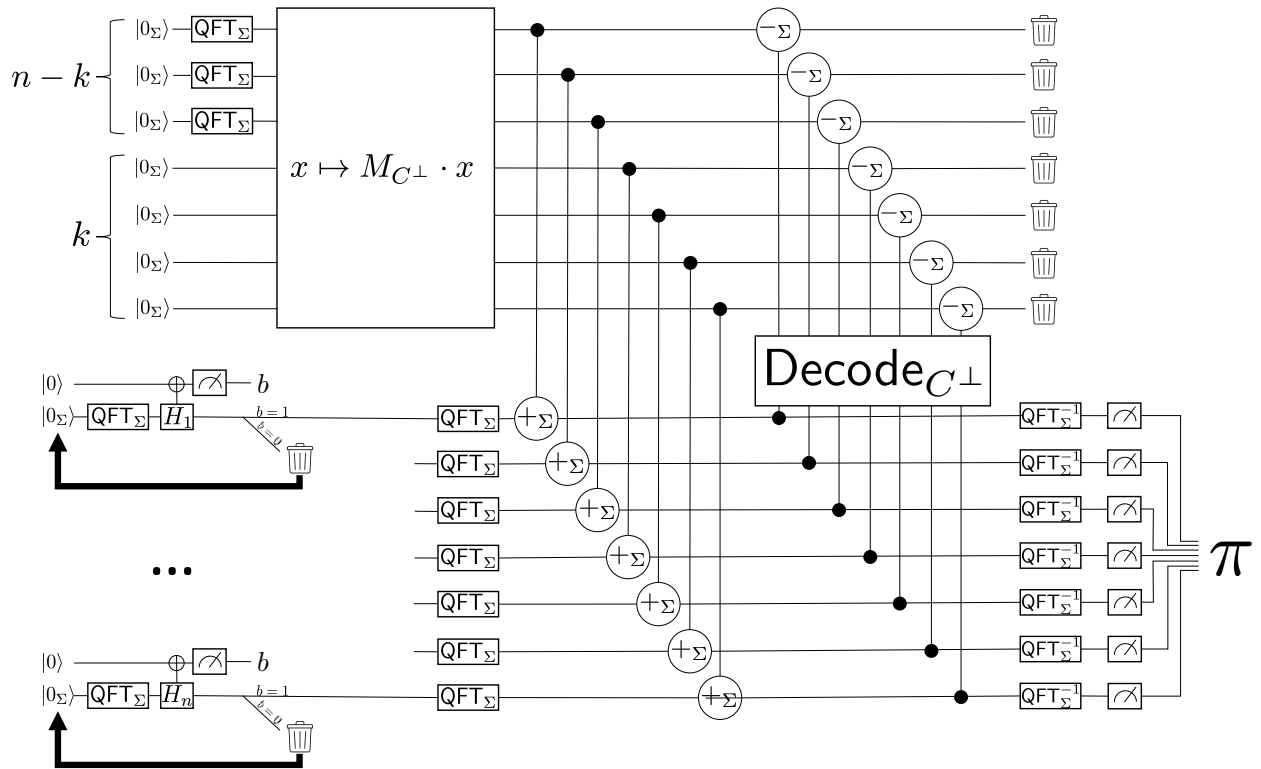
Figure 1: The algorithm Prove for computing \pi . Here, n - k is the rank of C^\perp , and M_{C^\perp} is any invertible matrix whose first n - k rows are a basis for C^\perp .
