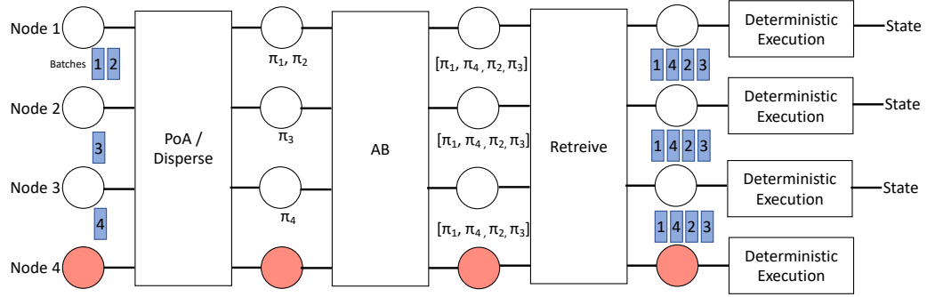
Fig. 1. Overview of the Layered SMR approach
