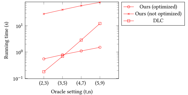
Figure 10: Running time of our approach and DLC with an increasing number of oracles. We fix security parameter to 40 and number of outcomes to 100. The y-axis is in log scale.
