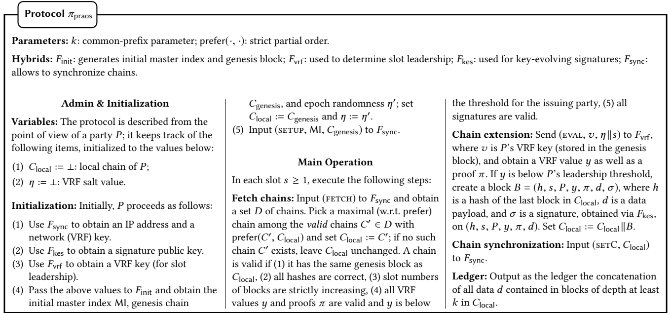
Figure 6: Protocol \pi_{\text{praos}} .
